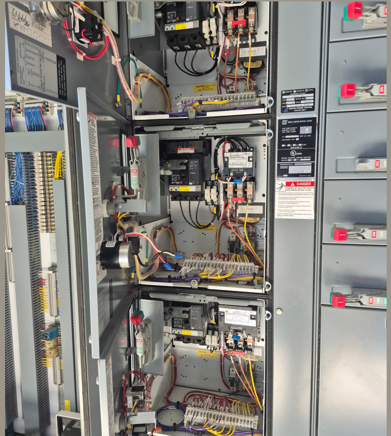
Troubleshoot and corrected BWR Pump #1 at the JLWTP trip issue
