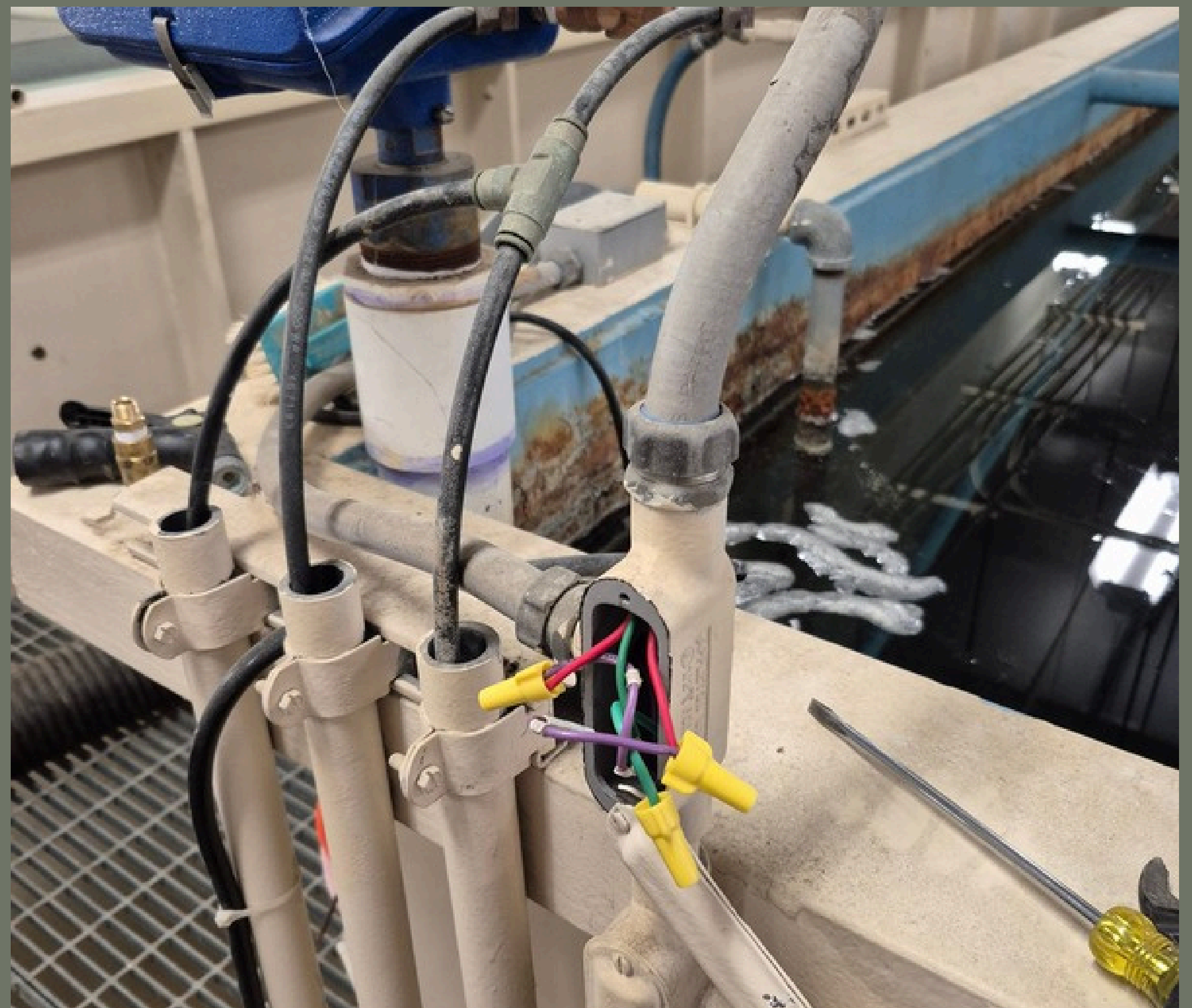
Electrical - Prepping Filter 1 For Rehab - Copper Cove
