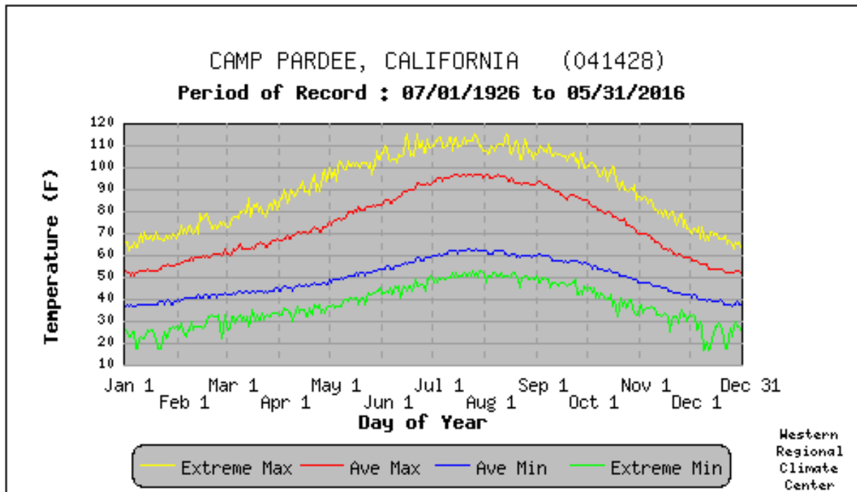
Figure 4-23 Daily Temperature Averages and Extremes, Camp Pardee, 1926 to 2016
