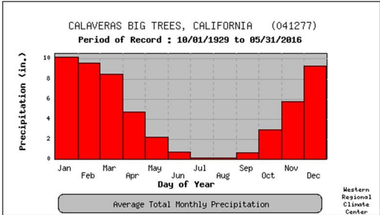
Figure 4-56 Calaveras Big Trees Monthly Average Total Precipitation, 1929 - 2016
