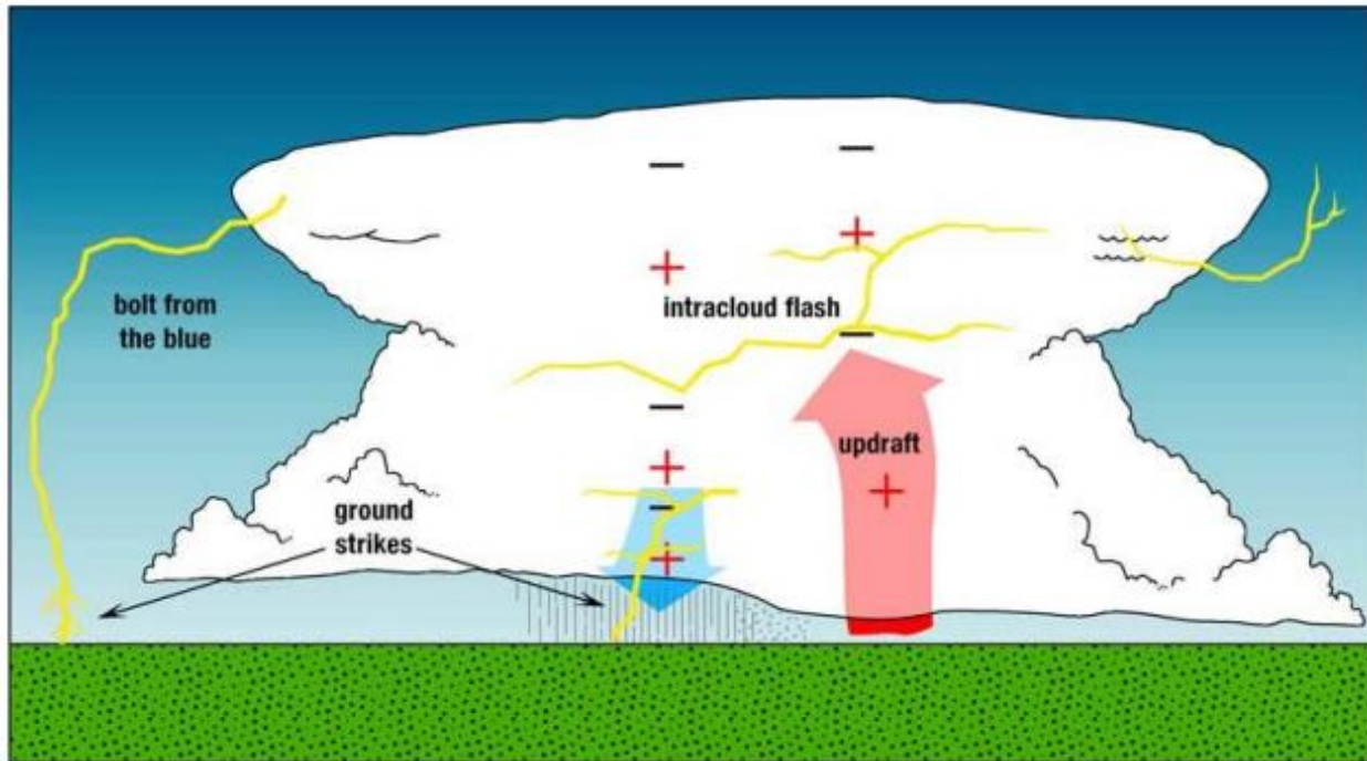
Figure 4-53 Cloud-to-Ground Lightning
