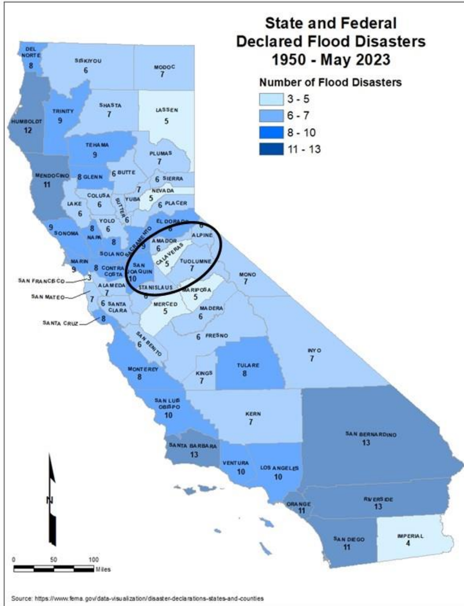
Figure 4-45: Calaveras County Flood Declarations from 1950 to 2023
