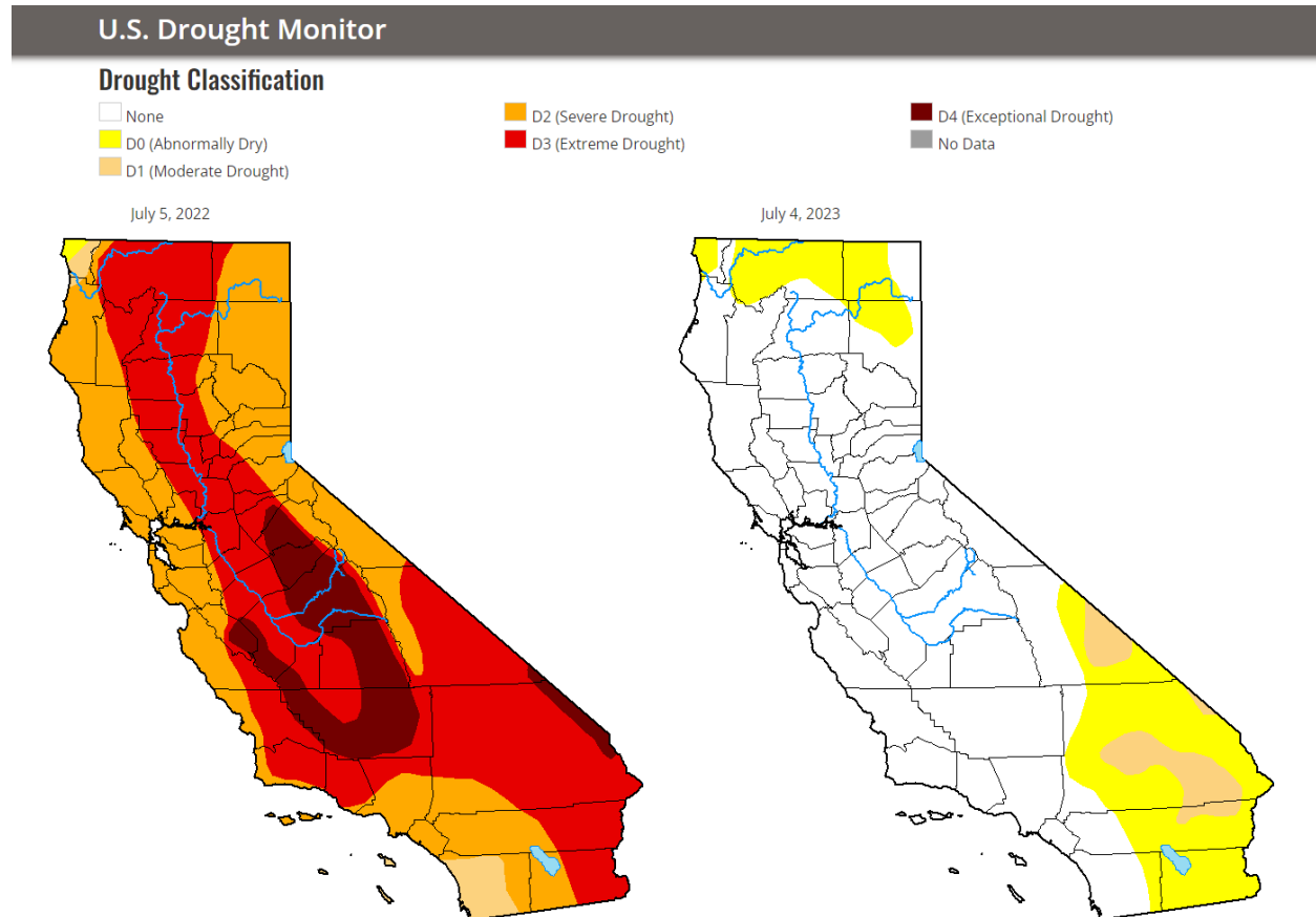
Figure 4-17 US Drought Monitor maps from July 2022 and July 2023
