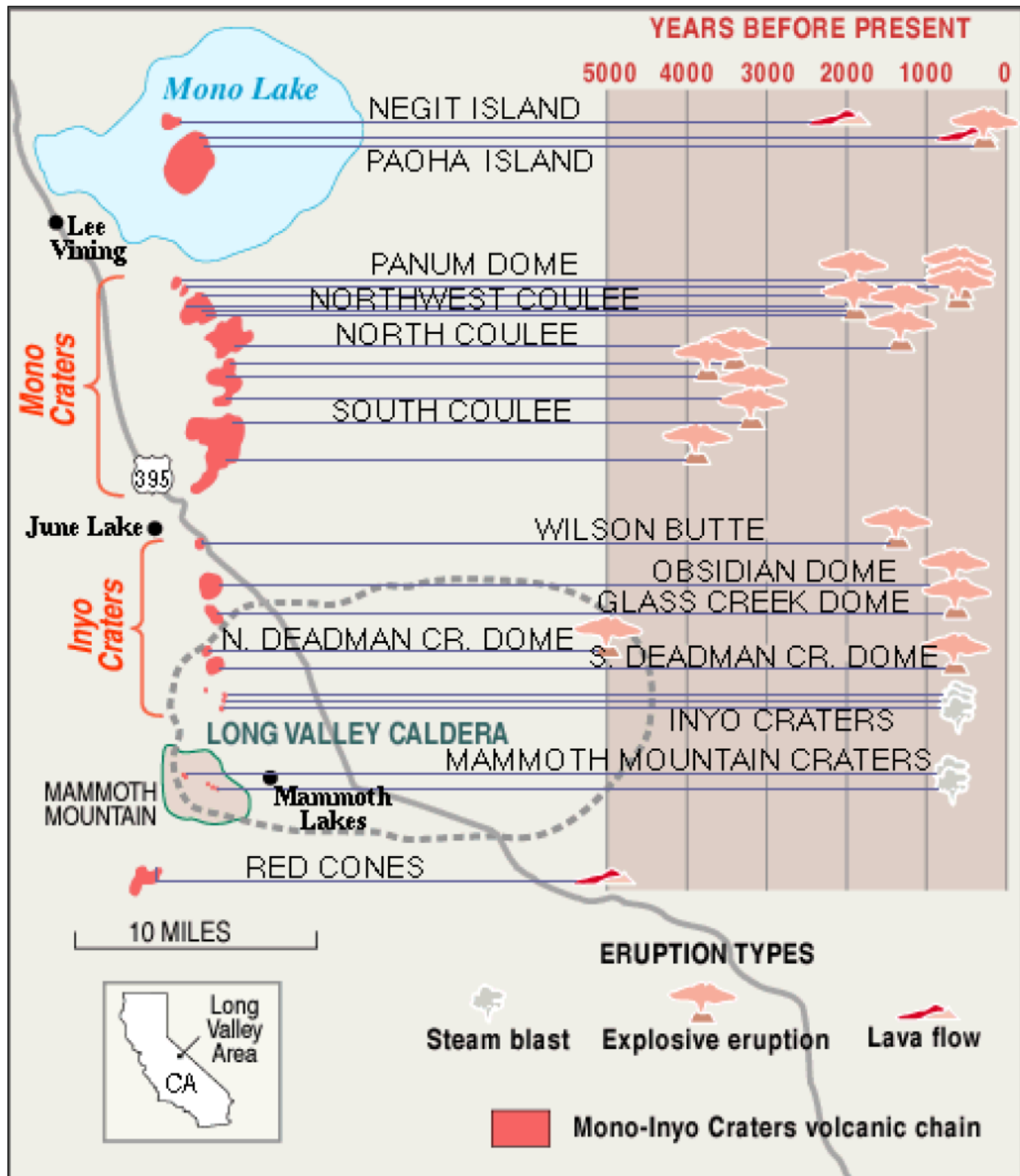
Figure 4-68 Volcanic Activity in the Mono-Inyo Craters Volcano Chain in the Past 5,000 Years
