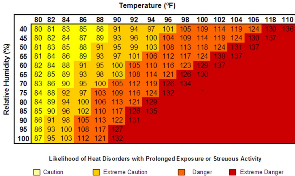
Figure 4-25 Heat Index
