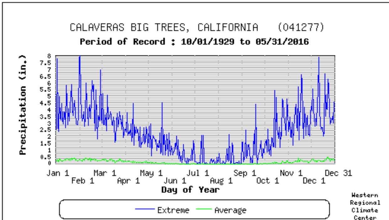
Figure 4-57 Calaveras Big Trees Daily Precipitation Average and Extremes, 1929 - 2016
