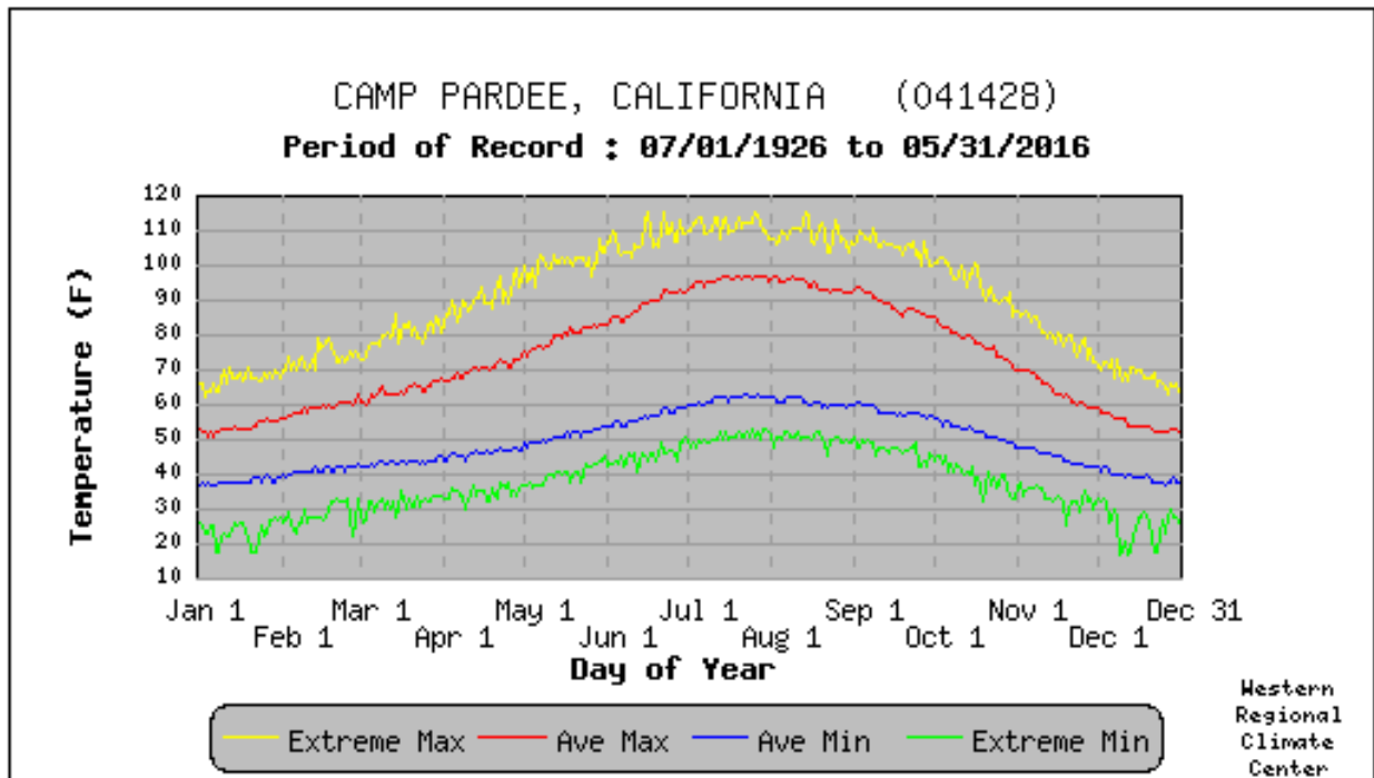
Figure 4-33 Daily Temperature Averages and Extremes, Camp Pardee, 1926 - 2016
