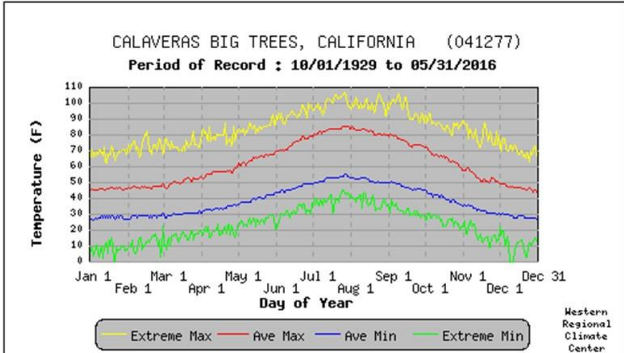
Figure 4-24 Daily Temperature Averages and Extremes, Calaveras Big Trees, 1929 - 2016
