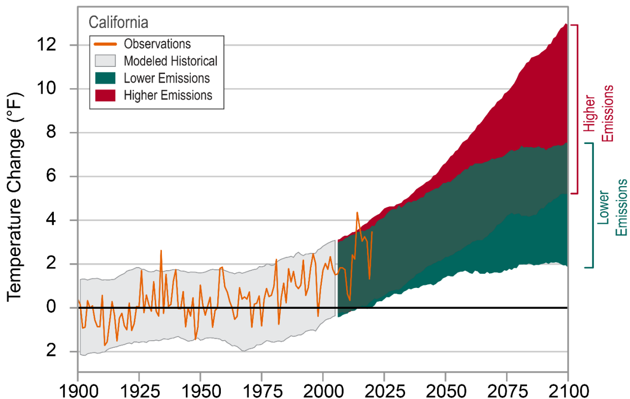
Figure 4-16 California Observed and Projected Temperature Change
