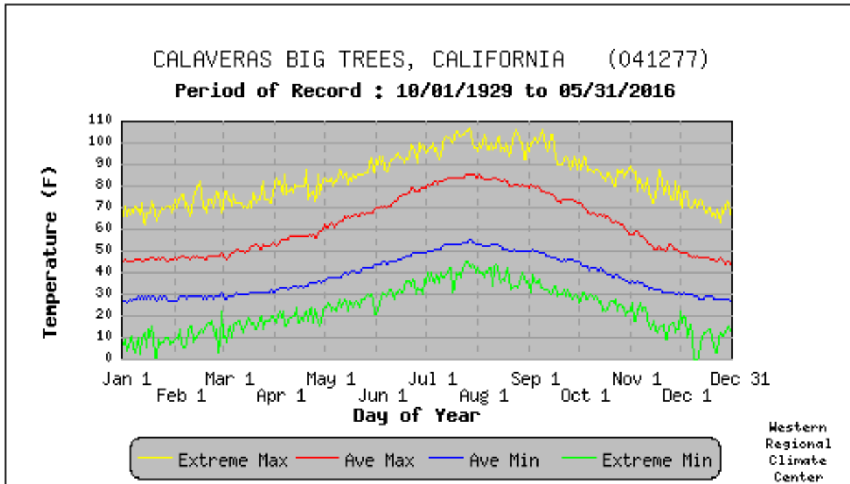
Figure 4-34 Daily Temperature Averages and Extremes, Calaveras Big Trees, 1929 - 2016
